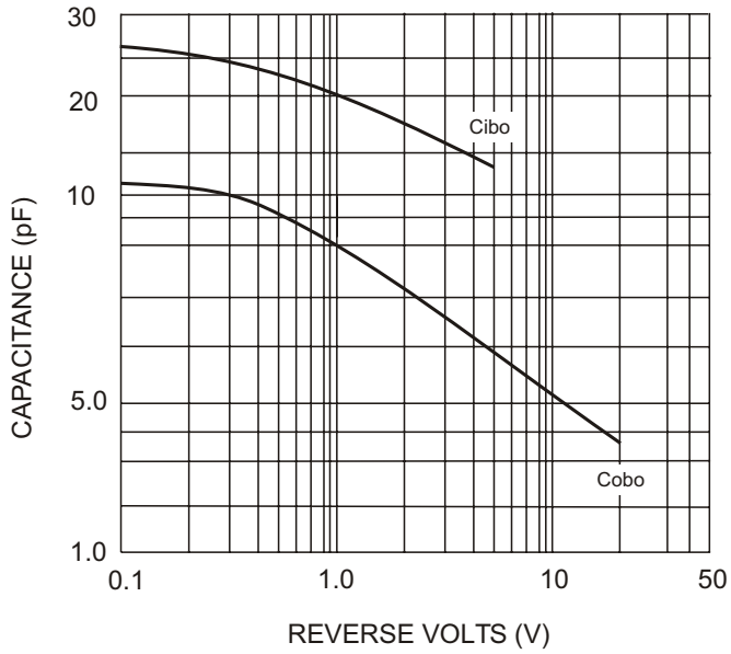
Fig. 1 Typical Capacitance
